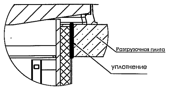
DETAIL E SCALE 1:15
